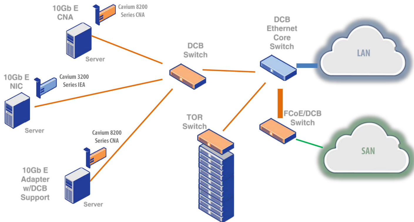
Figure 2. Data Center Bridging
